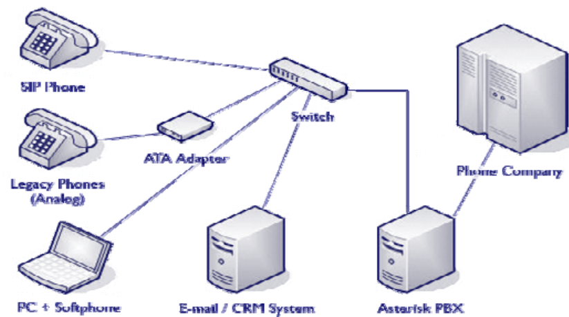
Figure 1: Asterisk Setup
