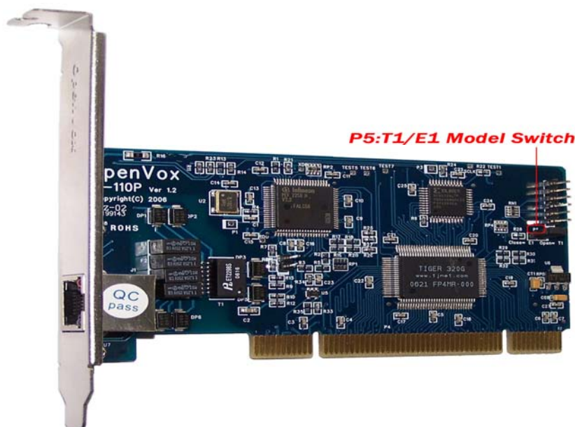
Figure 2: D110PG/D110P/D110E Hardware Configuration
